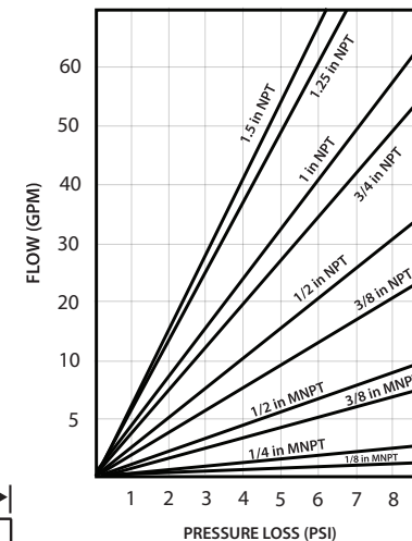
1/8 IN MNPT THRU 1.5 IN NPT INLINE STRAINERS
